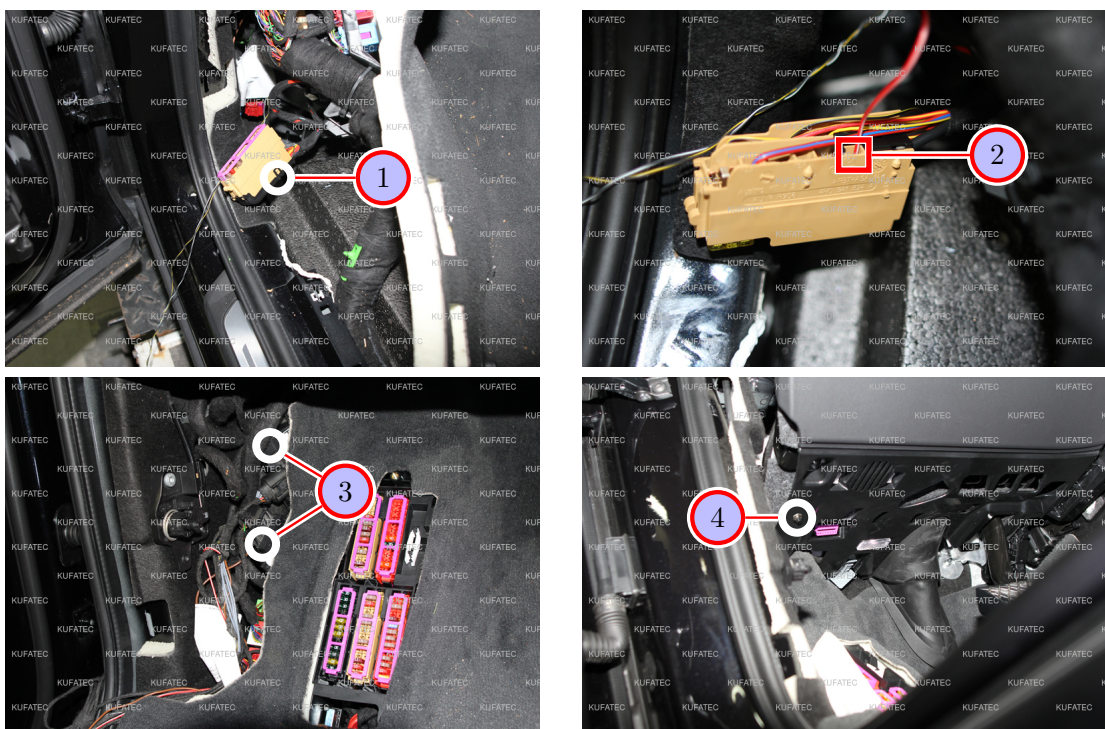
Figure 8: Connection ignition lead / installation pushbutton
