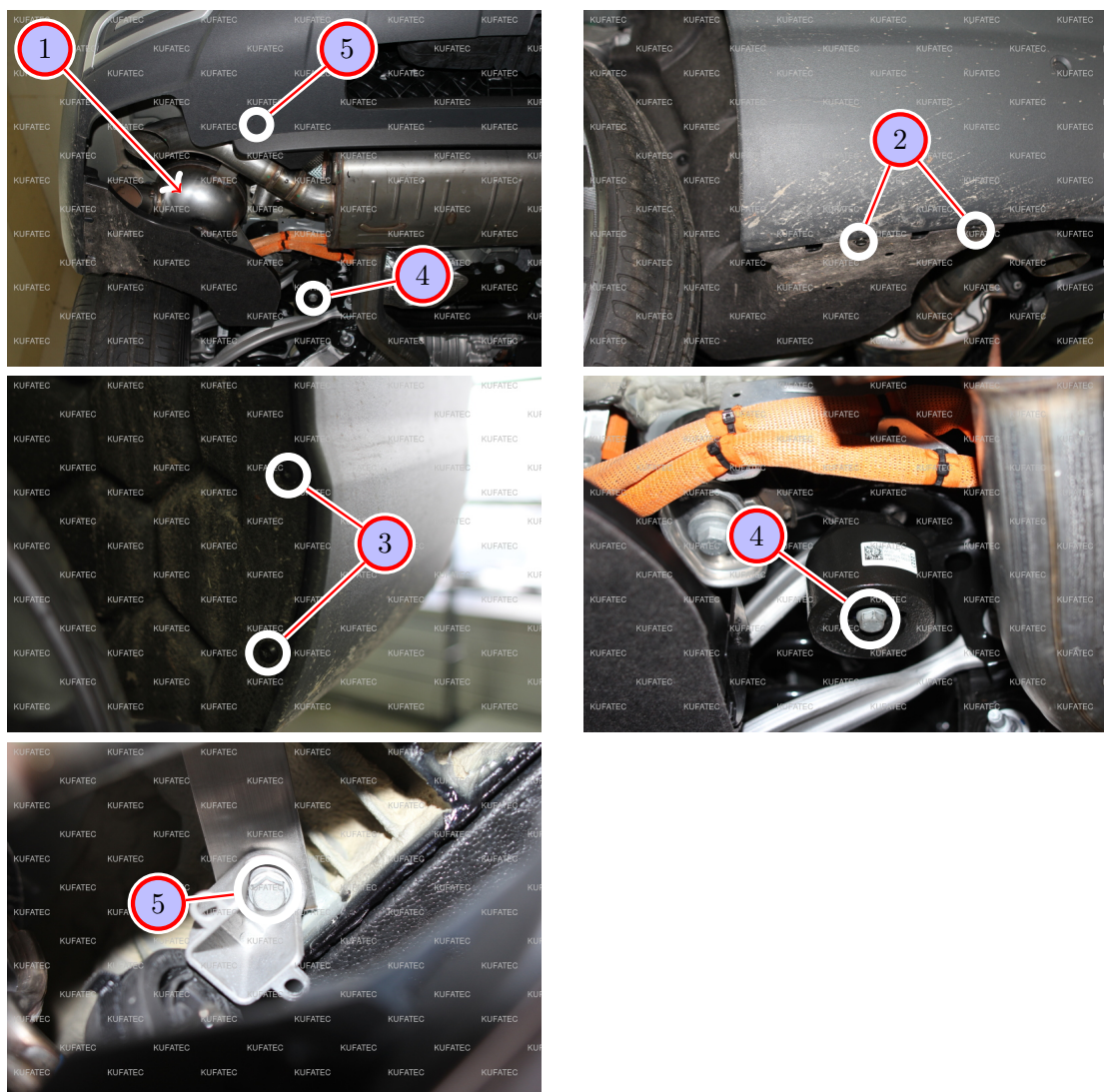
Figure 15: Installation sound generator
