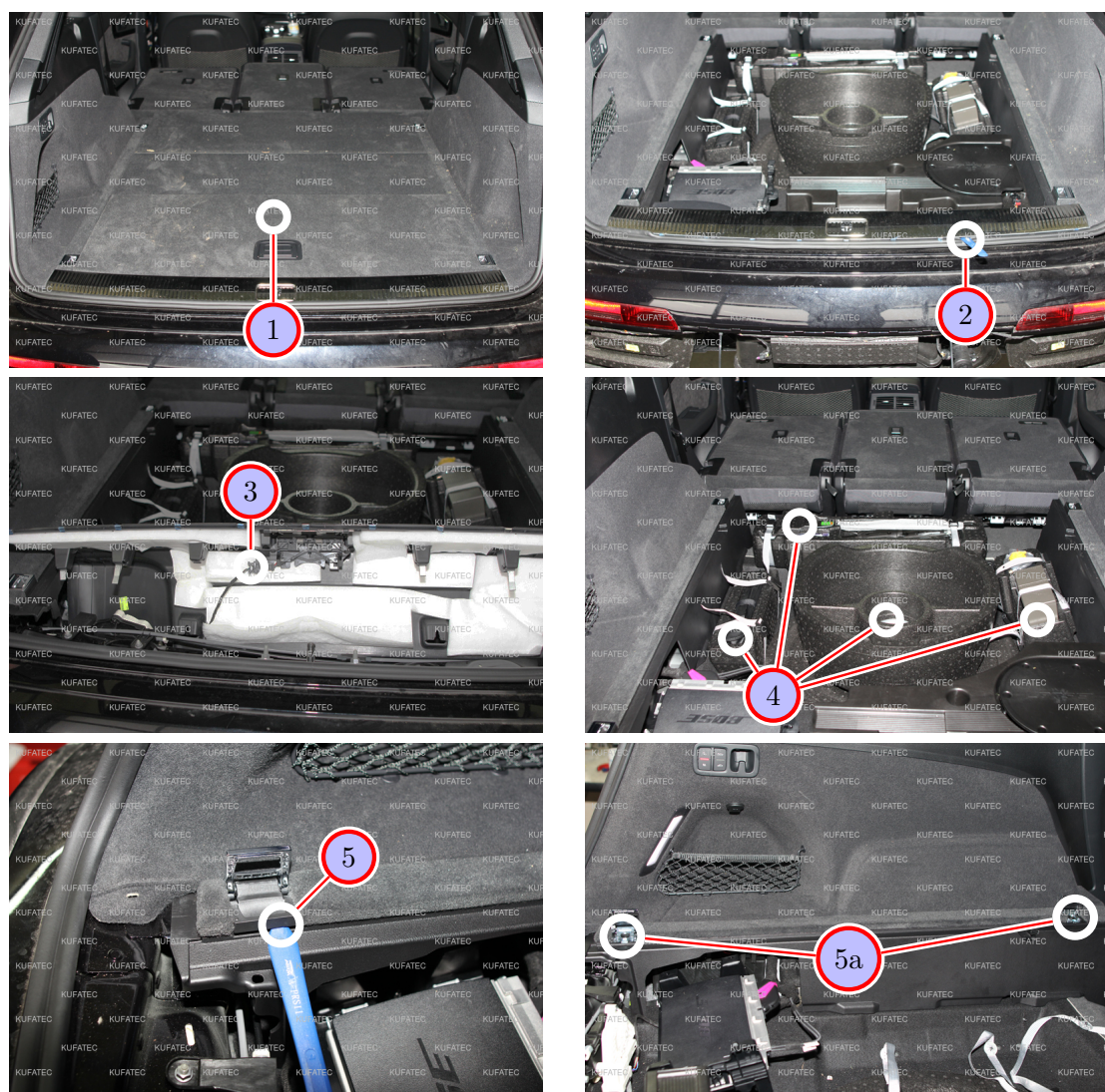
Figure 9: Disassembly left side covering trunk
