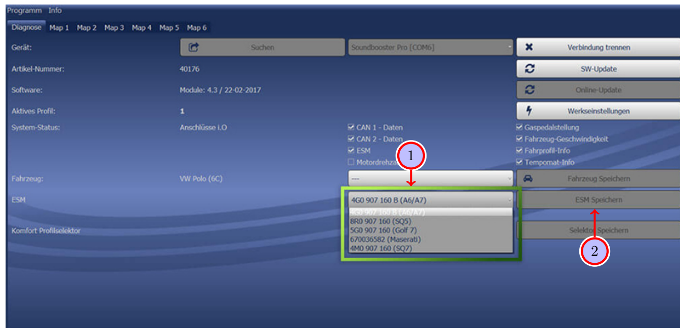
Figure 19: Software
