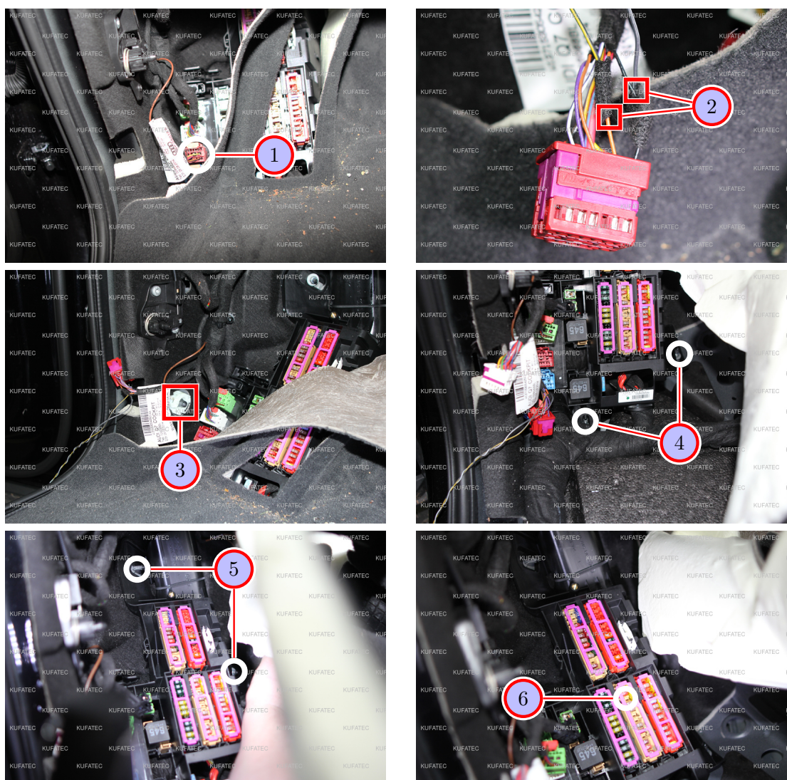
Figure 6: Connection Can High & Low / Ground (Variant prefacelift Model)
