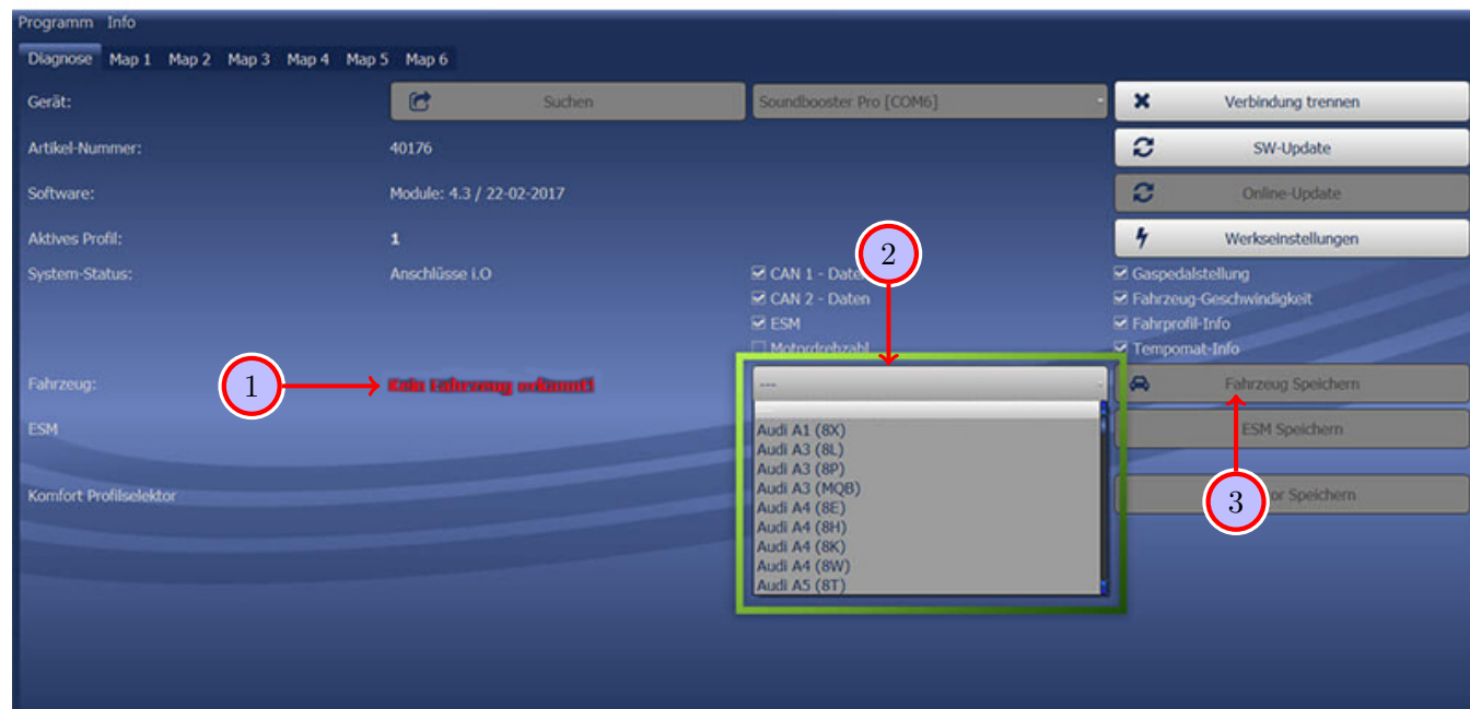
Figure 18: Software
