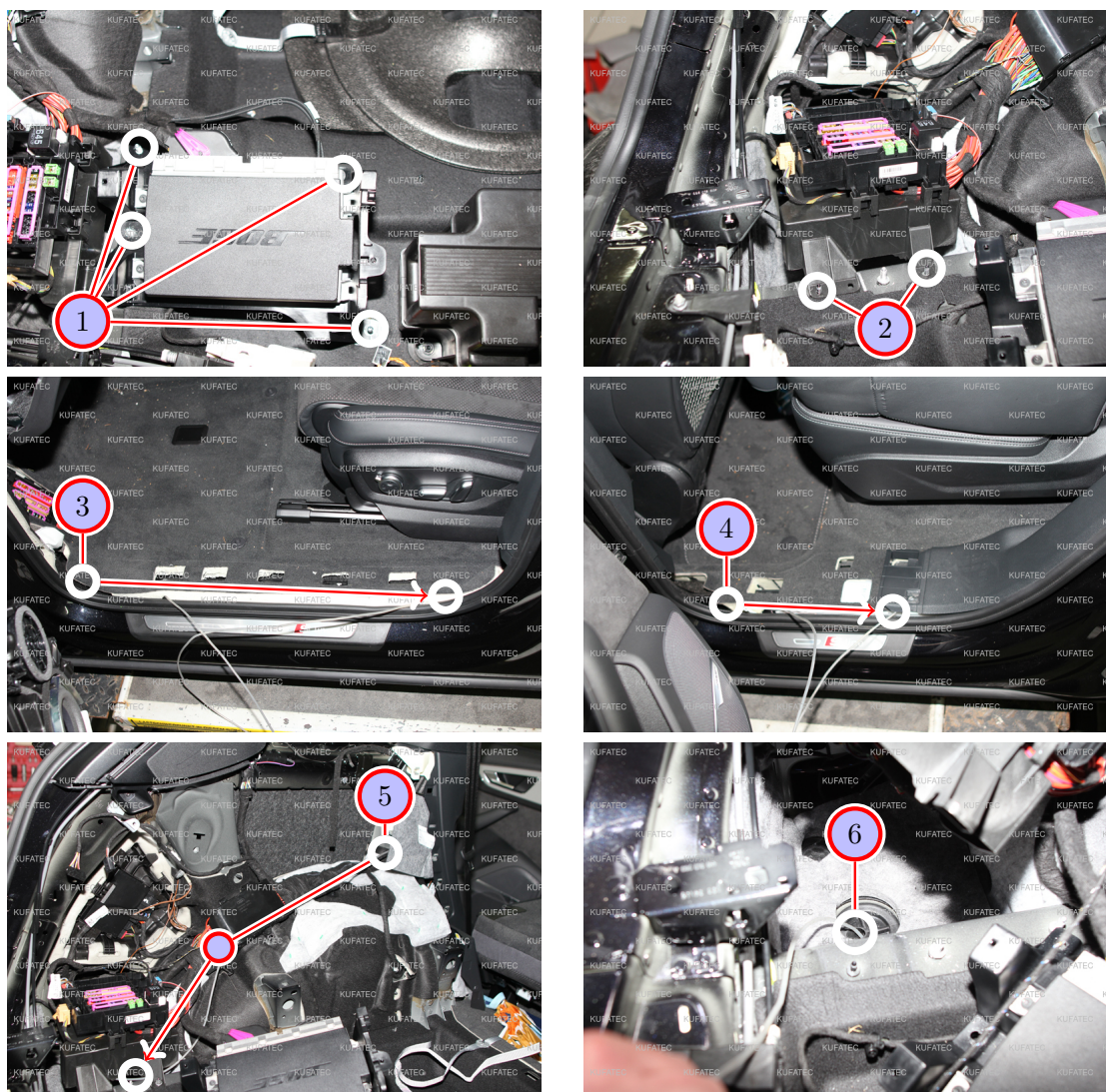
Figure 11: Removing fuse box trunk / cable routing
