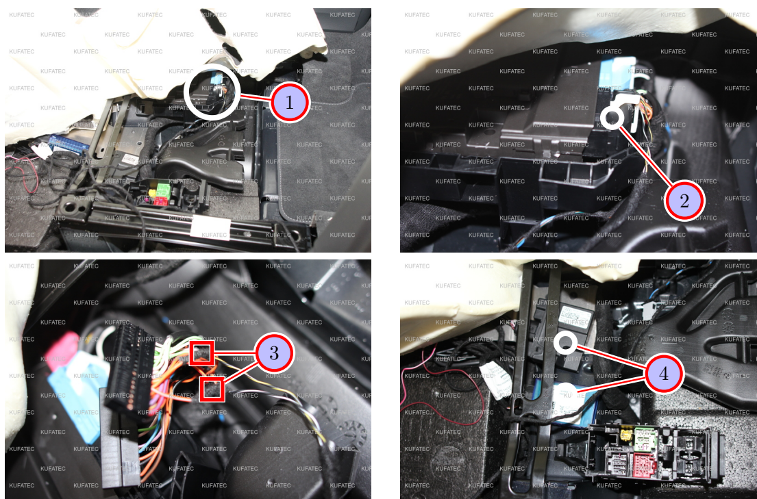
Figure 7: Connection Can High & Low / Ground (Variant Facelift Model)
