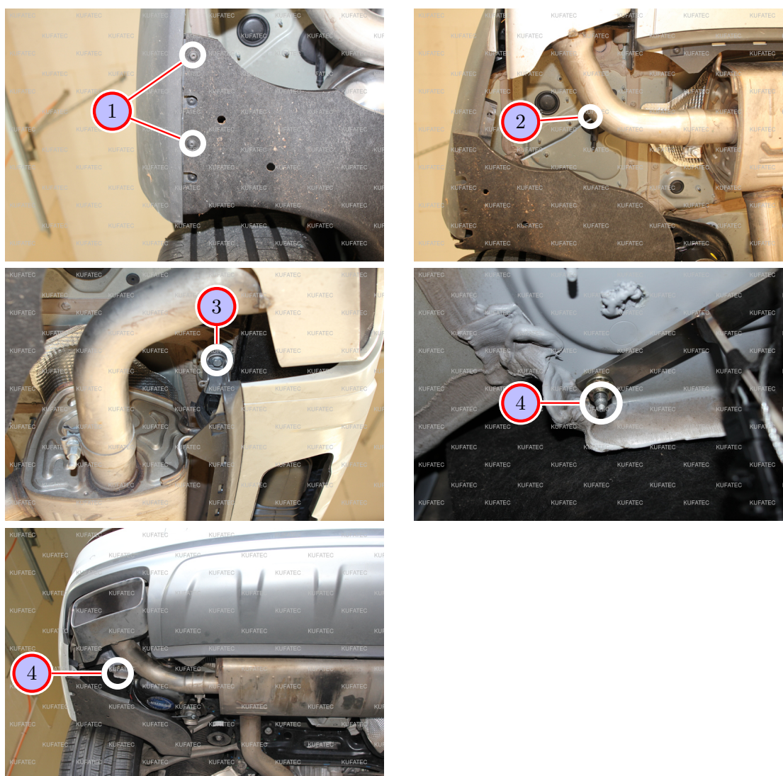
Figure 12: Installation sound generator
