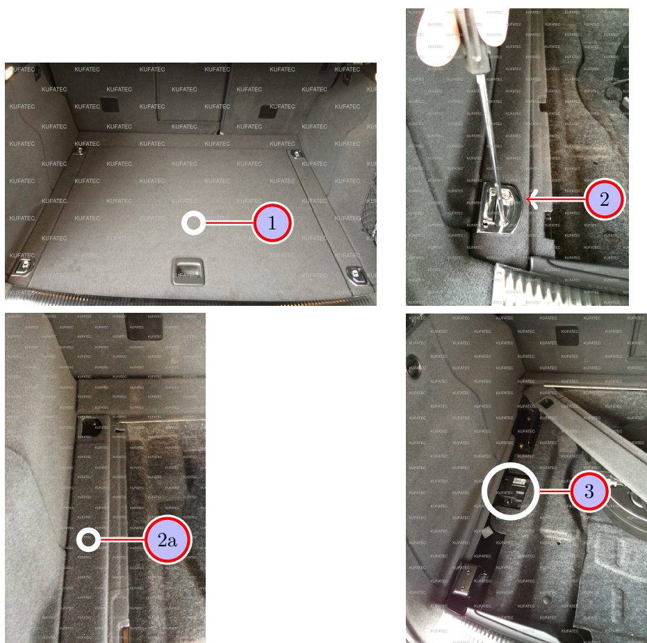
Figure 5: Installation instructions for Audi Q5 8R
