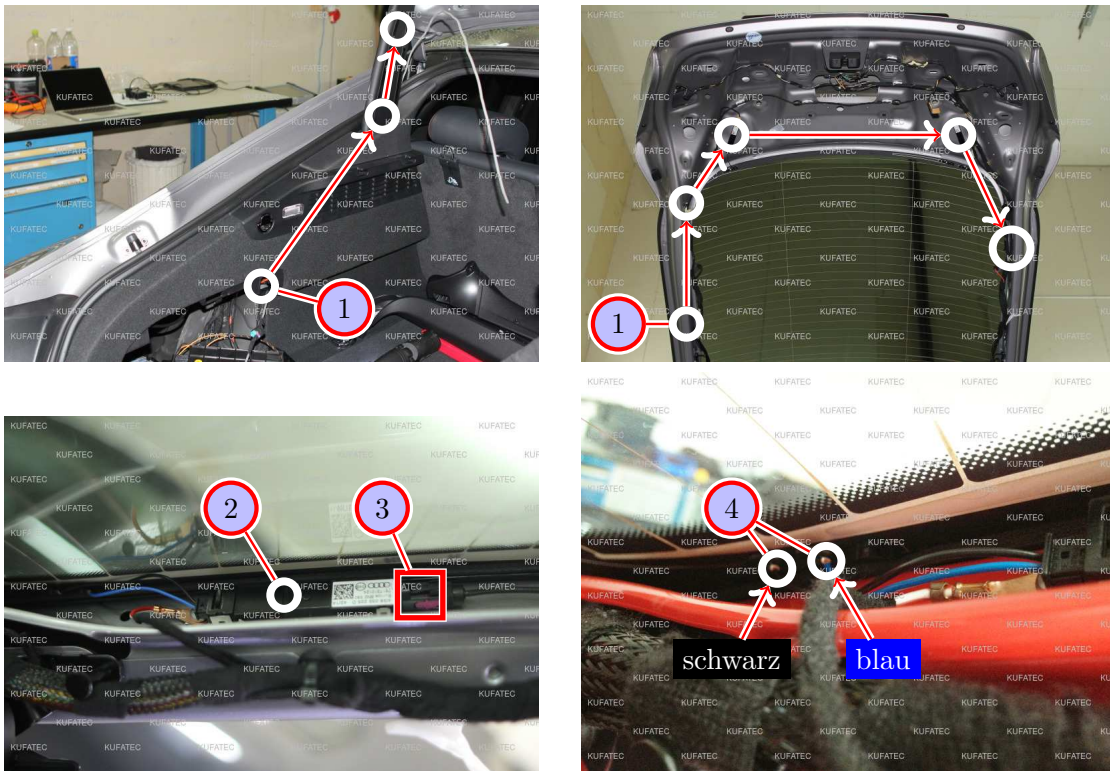
Figure 5: Installation / Connection Antenna Module
