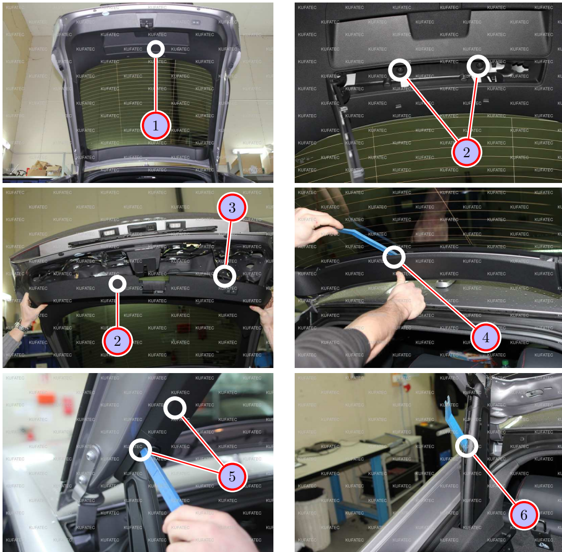
Figure 4: Pictures Removal Tailgate Covering
